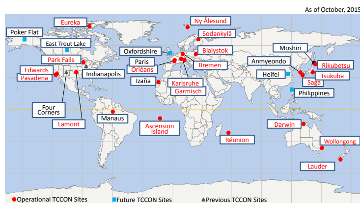
Figure 25. Sounding locations of the ground-based high-resolution Fourier transform spectrometers in the Total Carbon Column Observing Network. Sites shown in red have been used for the data validation.
