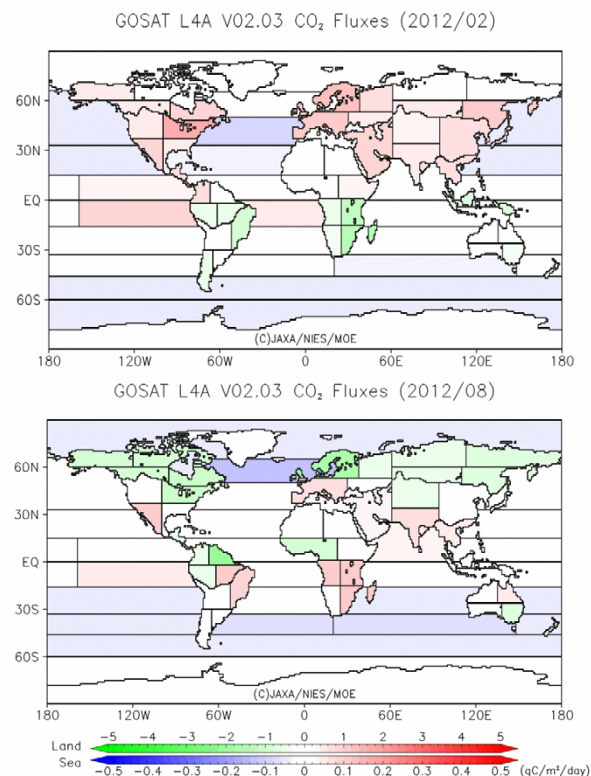
Figure 5. Sample estimates of global \text{CO}_2 sources and sinks ( \text{gC}/\text{m}^2/\text{day} ). February (upper), August (lower), 2012.
