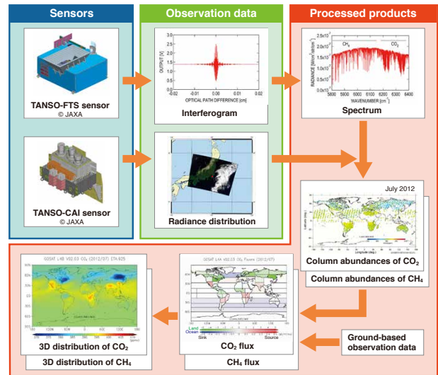
Figure 7. Outline of GOSAT data processing.
