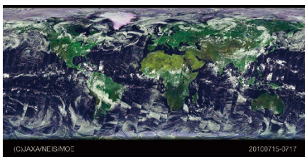
Figure 18. CAI Level 3 global radiance distribution obtained between July 15 and 17, 2010.
