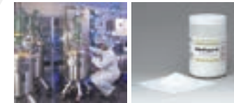
Oligonucleotide API contract manufacturing Particles for Nucleic Acid Synthesis
