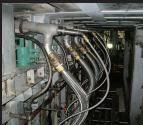
溶解槽燃焼器 Burner of Melter
